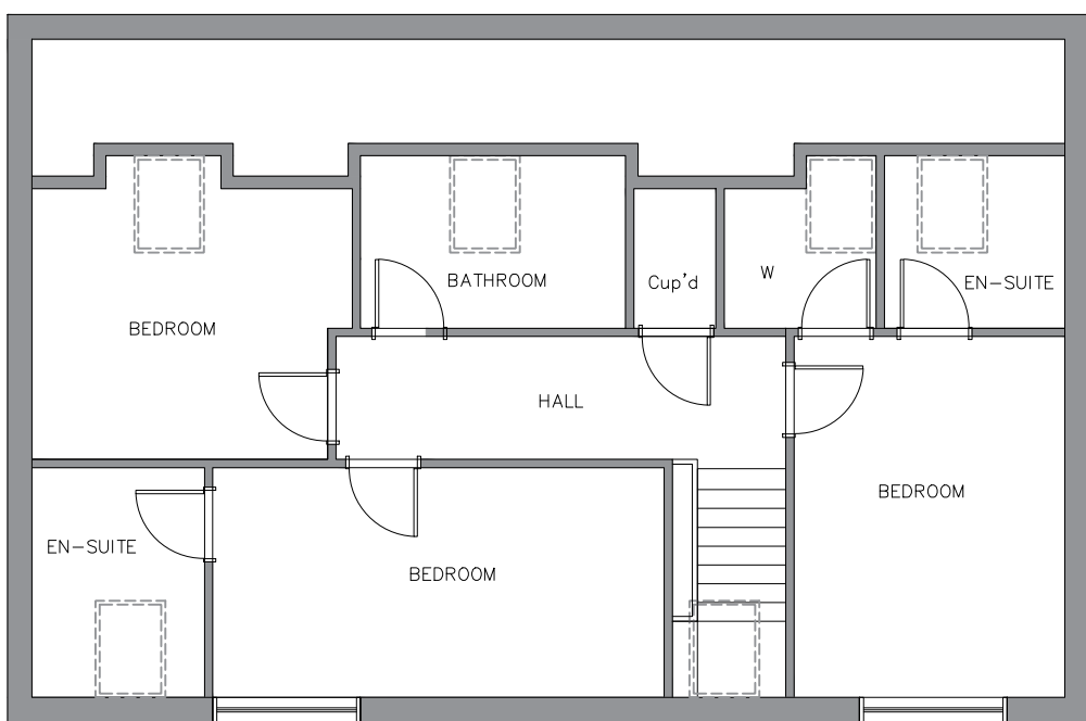
FIRST FLOOR PLAN – PROPOSED
