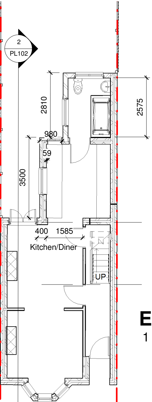
Existing Ground Floor Plan NH
