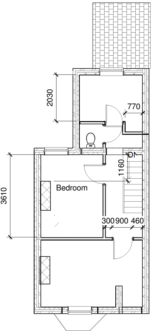
Existing First Floor Plan NH
