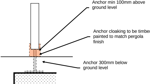
Anchor Detail
