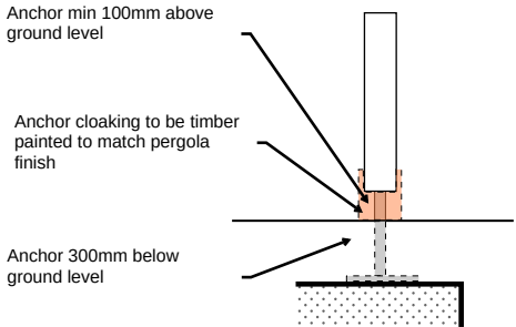
Anchor Detail
