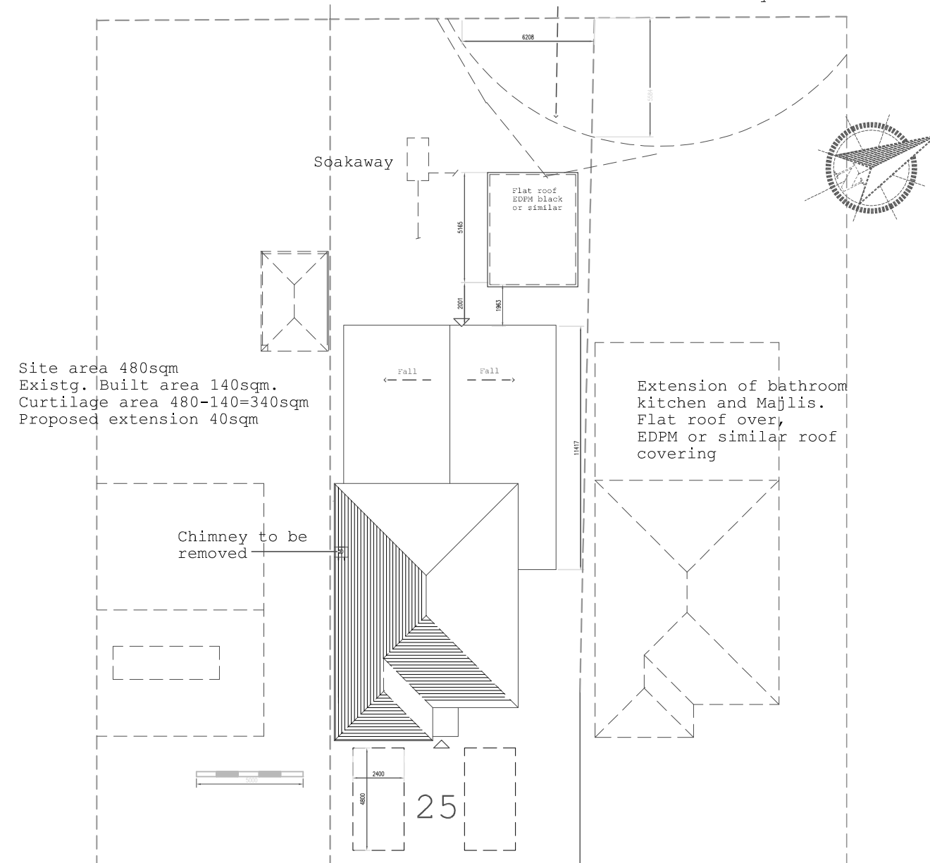
25 Clifton Gardens Existing Roof Plan
