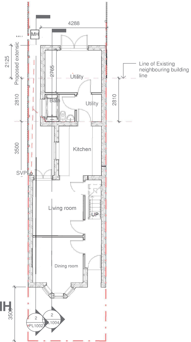
Proposed Ground Floor Plan NH 1 : 100
