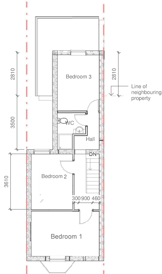
Proposed First Floor Plan NH 1 : 100
