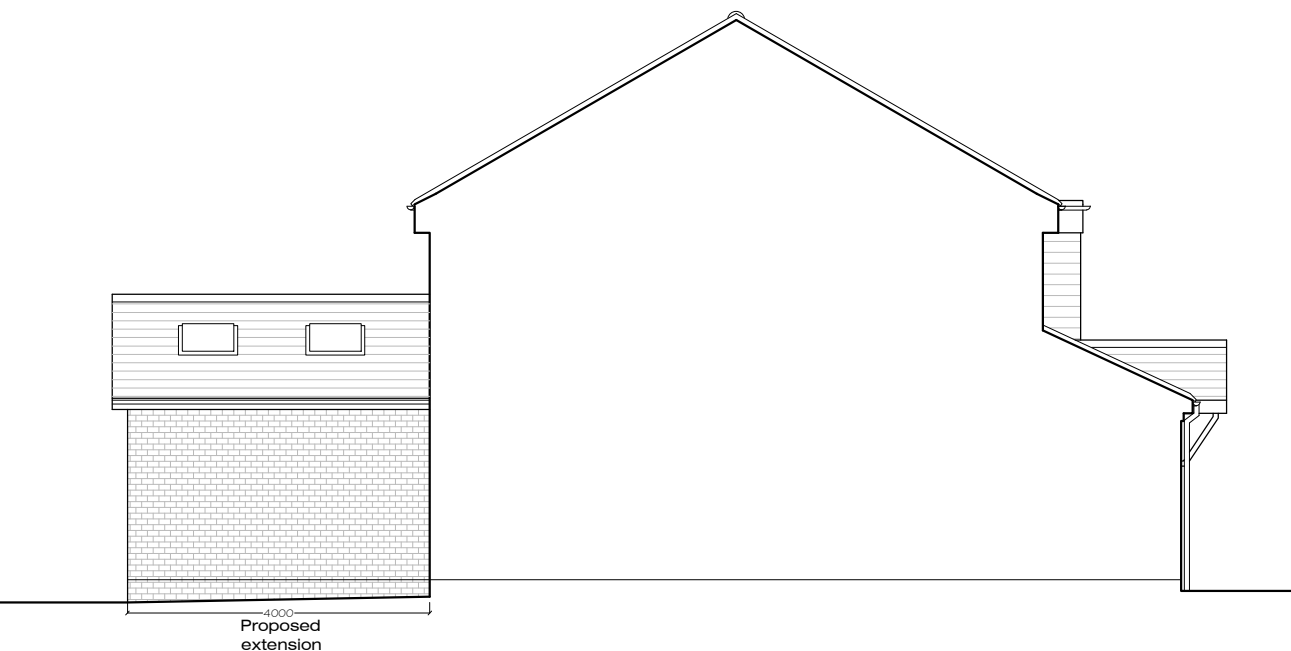
North-East (Side) Elevation - As Proposed
