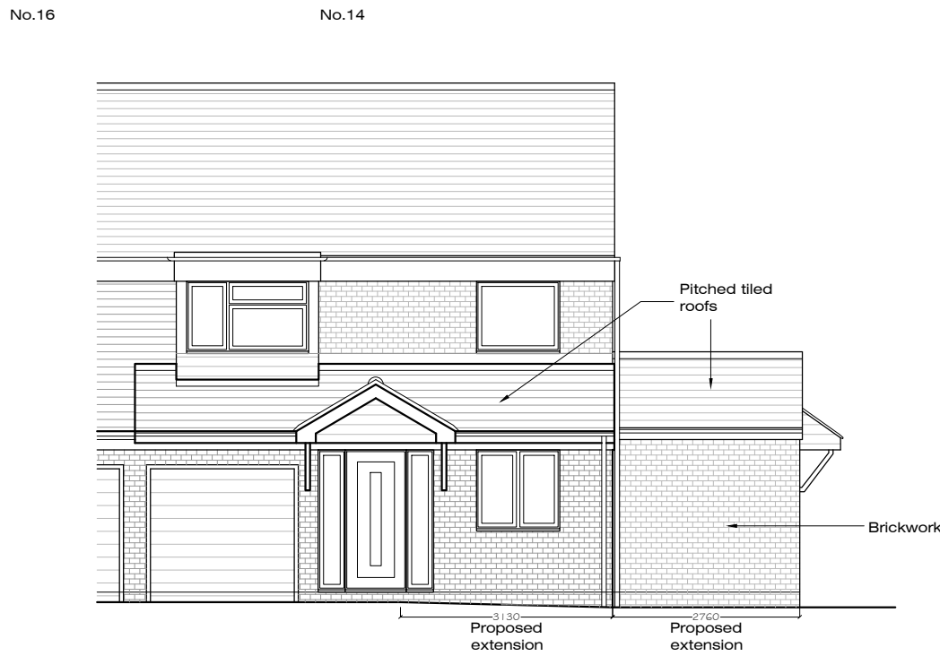
North-West (Front) Elevation - As Proposed
