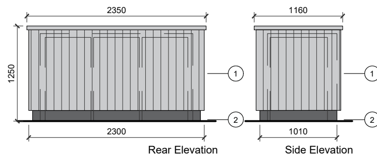
Rear Elevation
