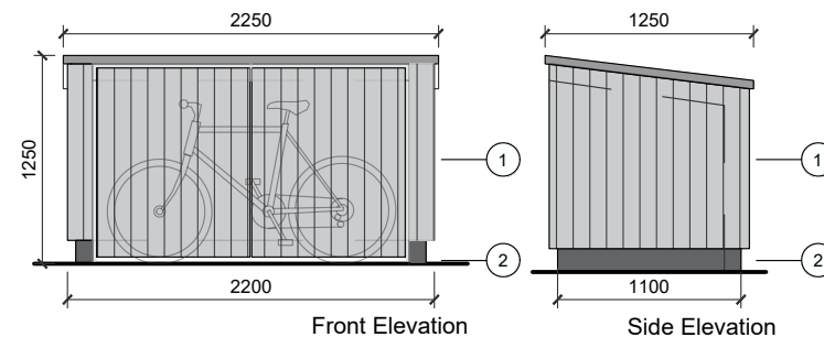
Front Elevation
