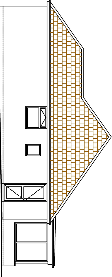
EXISTING NORTH ELEVATION 1:100
