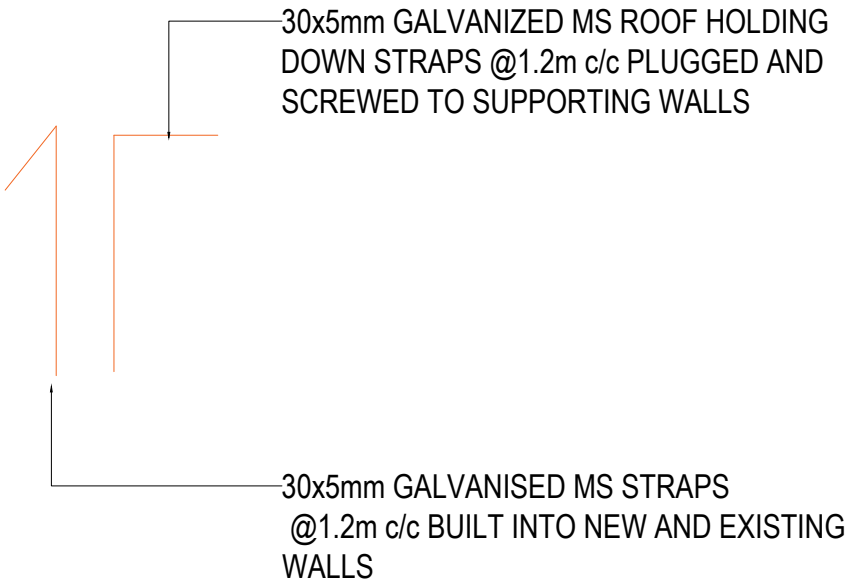
Lateral Strap
