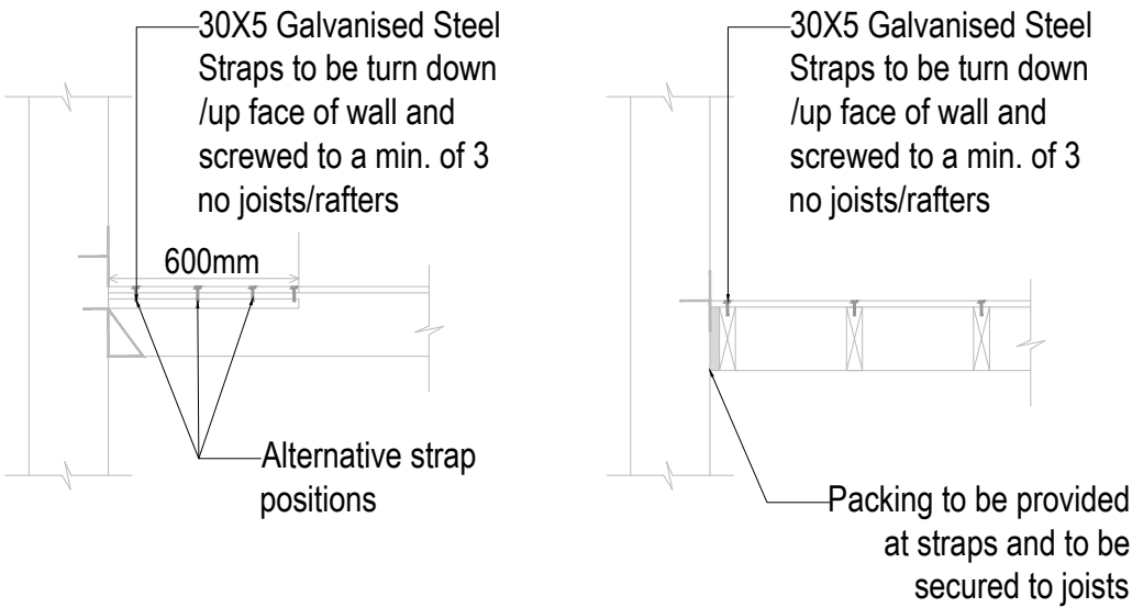
Joists Perpendicular To Wall
