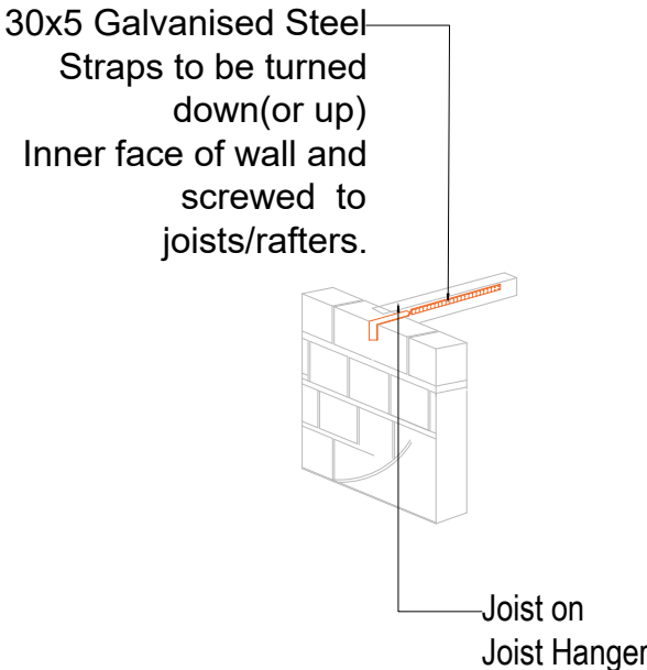
Strap Detail For Wall
