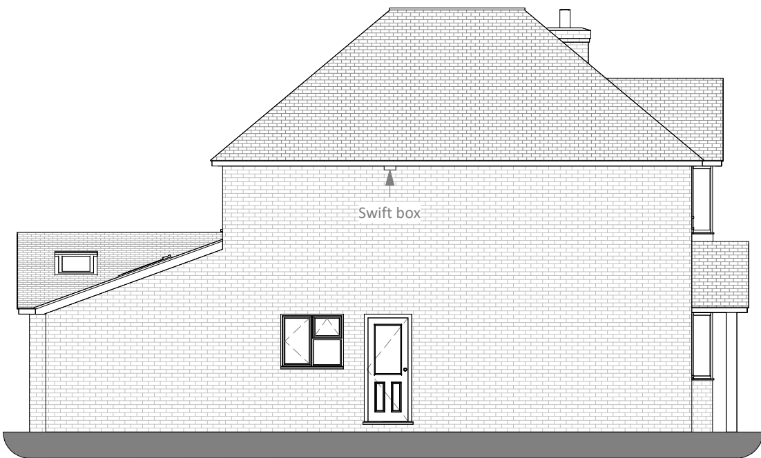
8 Proposed NE Elevation 1 : 100
