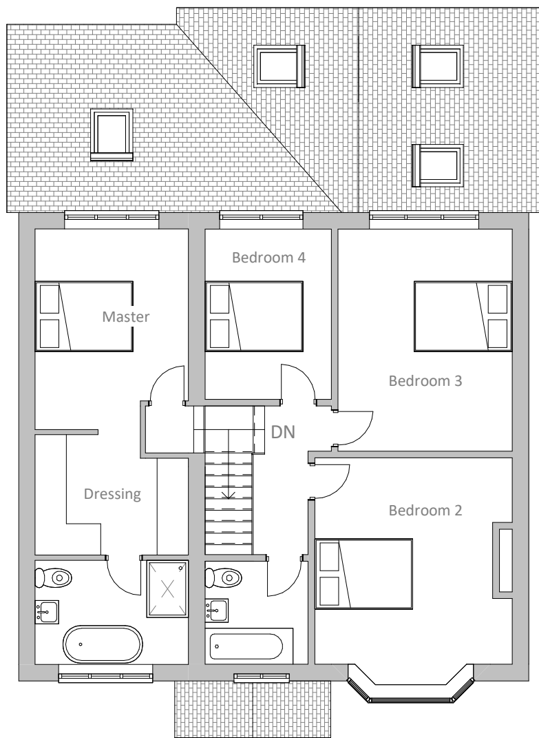
12 Proposed First Floor Plan 1 : 100
