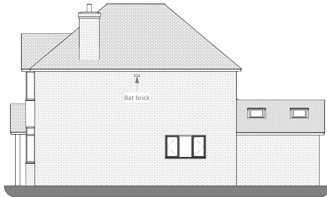
10 Proposed SW Elevation 1 : 100
