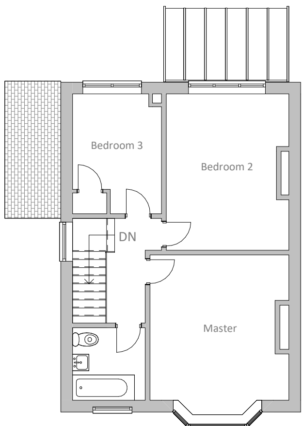
11 Existing First Floor Plan 1 : 100
