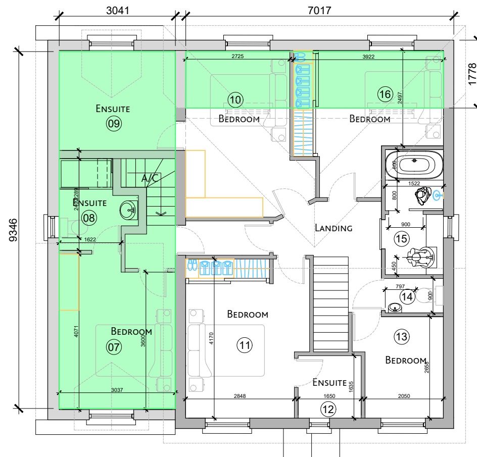
FIRST FLOOR -AS GRANTED UNDER APPROVAL 25/99460
