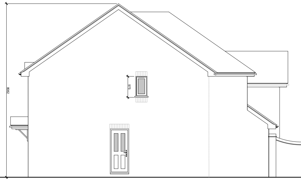
PROPOSED SIDE ELEVATION - AS APPLIED FOR UNDER SECTION 73 APPLICATION (VARY A CONDITION)
