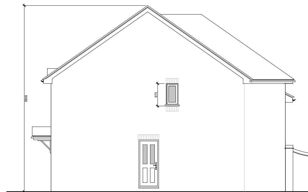
PROPOSED SIDE ELEVATION - AS GRANTED UNDER APPROVAL 25/99460
