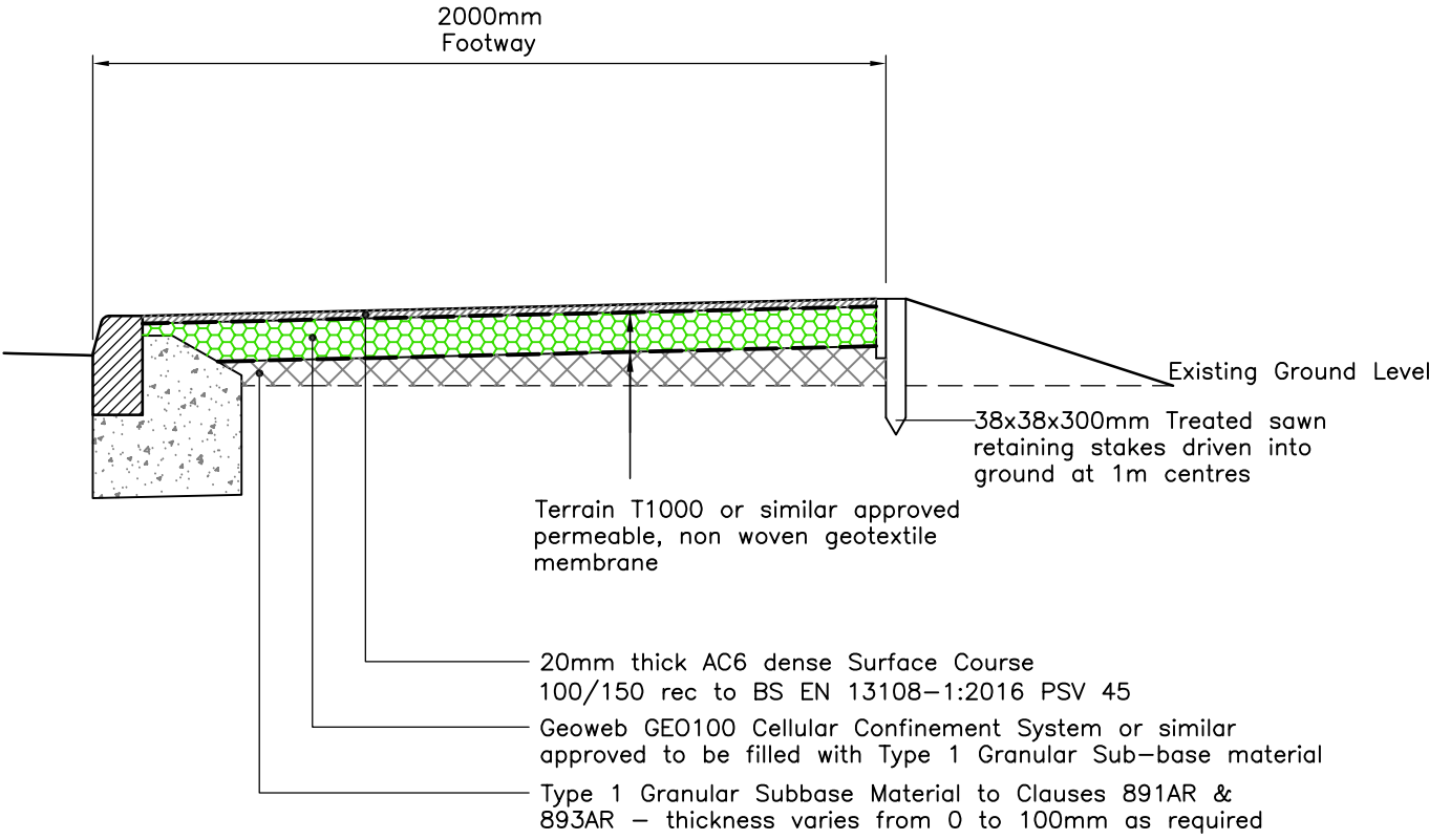
No Dig Footway Construction
