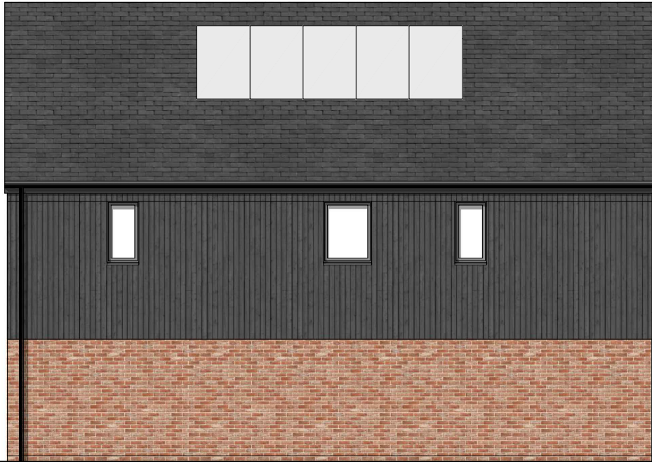
REAR elevation
