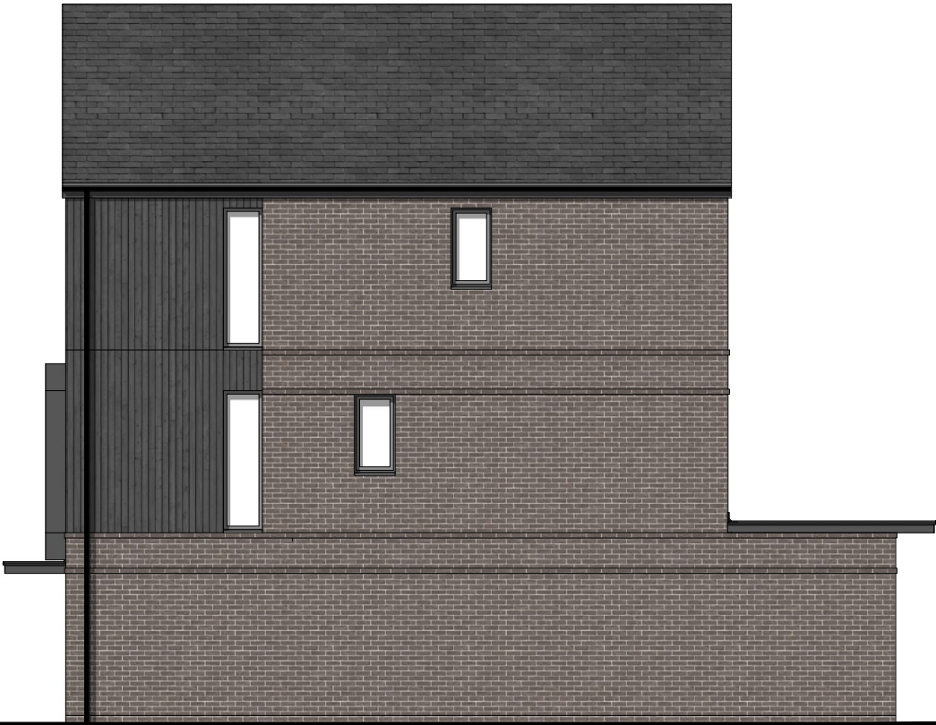
SIDE elevation
