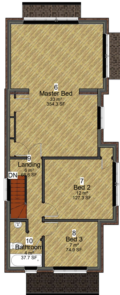
2 First Floor Plan 1 : 100
