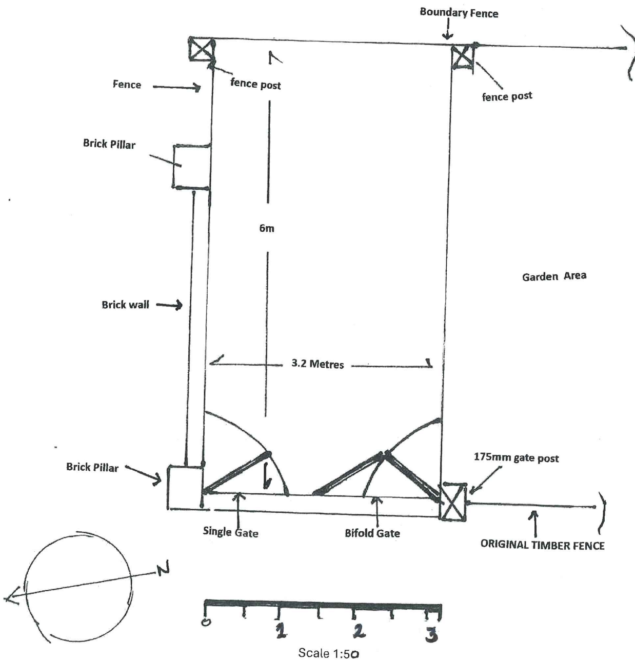
BLOCK PLAN OF GATE INSTALLATION
