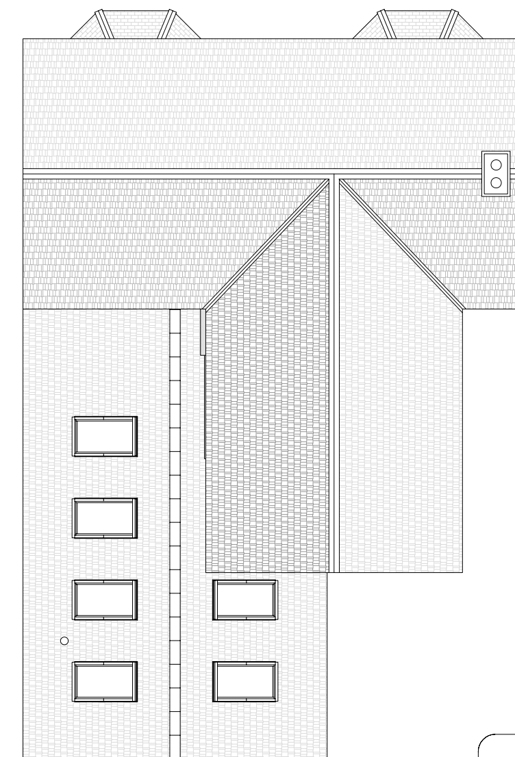
ROOF PLAN
