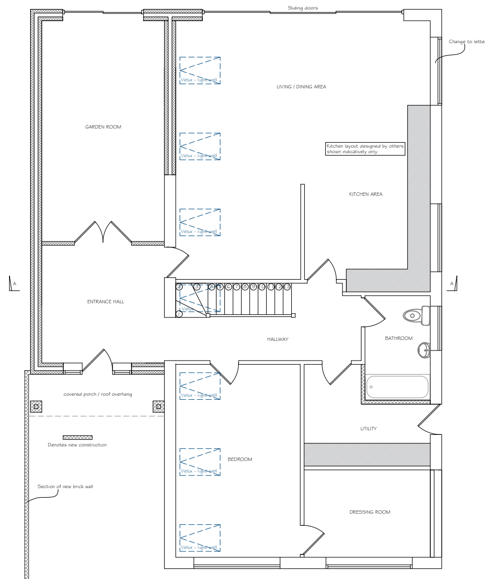
Proposed Ground Floor Plan 1:100 @ A3
