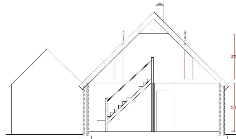
Proposed Section AA 1:100 @ A3
