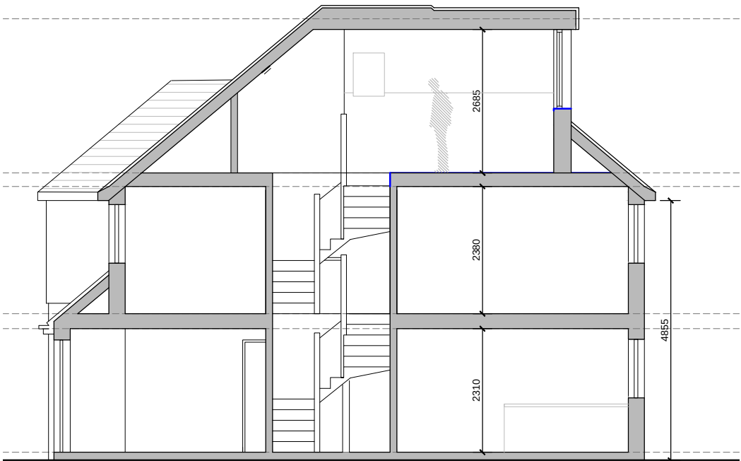
Building Section B-B
