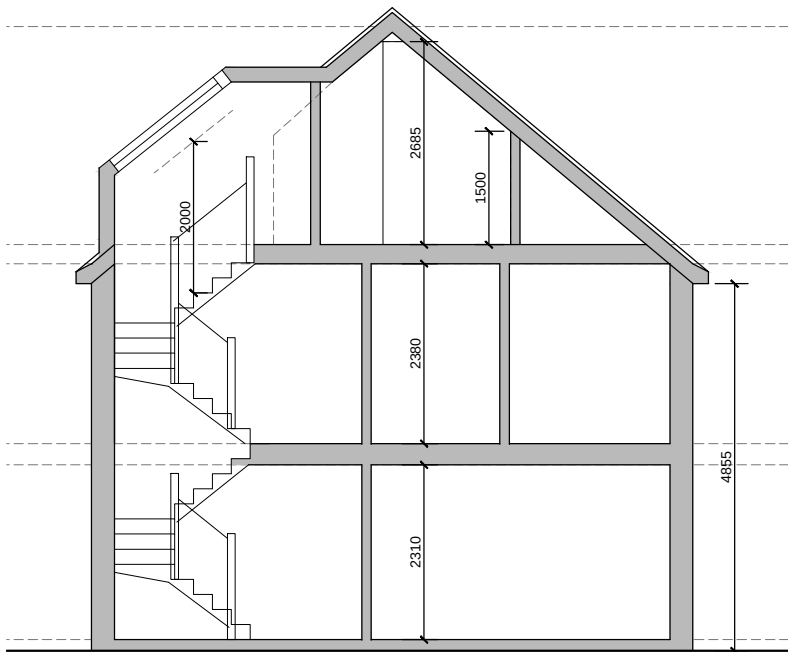
Building Section A-A
