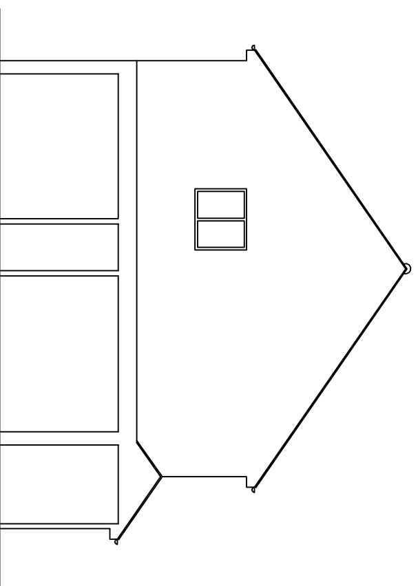
Left Elevation Proposed
