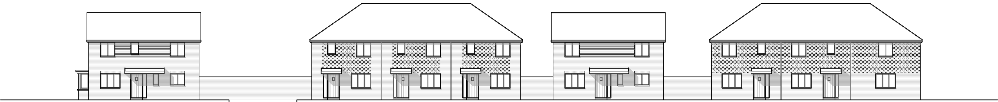
Street Scene F - F
