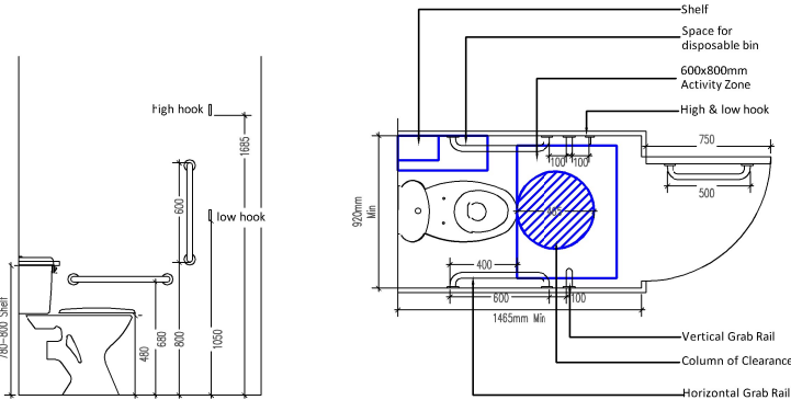
AMBULANT DISABLED TYPICAL CUBICLE SETTING OUT
