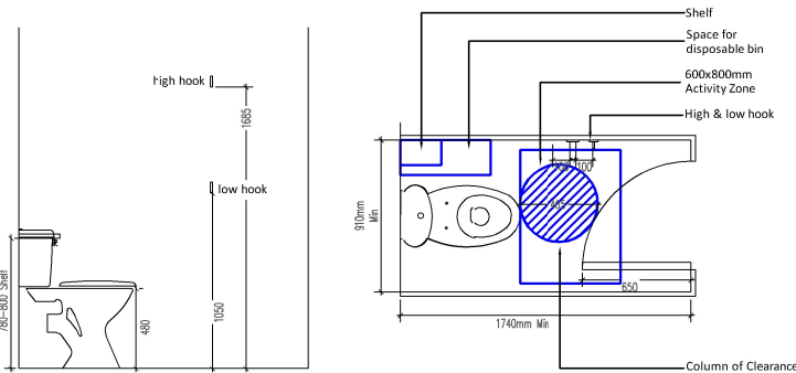
AMBULANT DISABLED TYPICAL CUBICLE SETTING OUT
