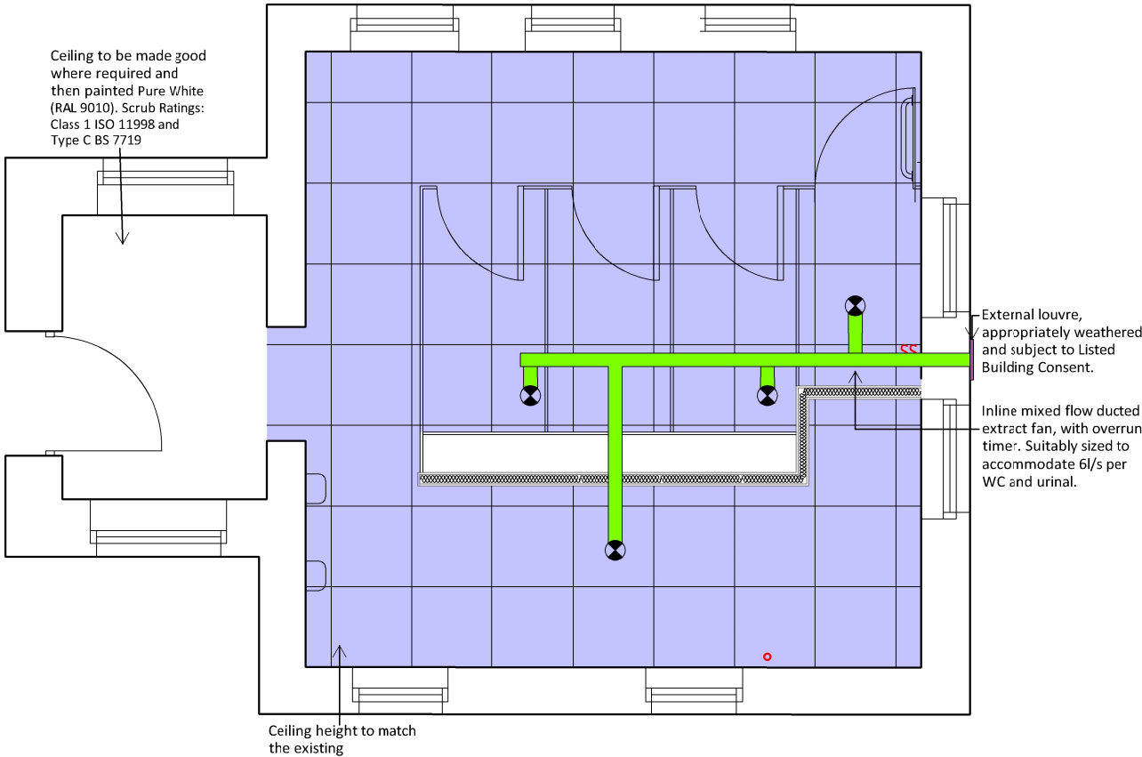
PROPOSED CEILING PLAN - 1-007 WC
