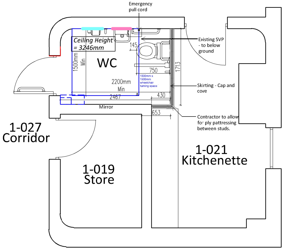
PROPOSED GENERAL ARRANGEMENT PLAN - 1-020 WC
