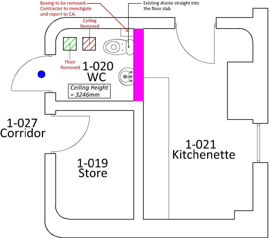
DEMOLITION AND ALTERATION - 1-020 WC
