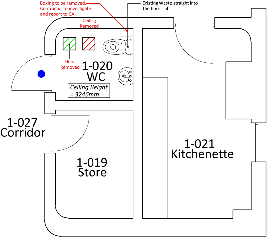
EXISTING PLAN - 1-020 WC
