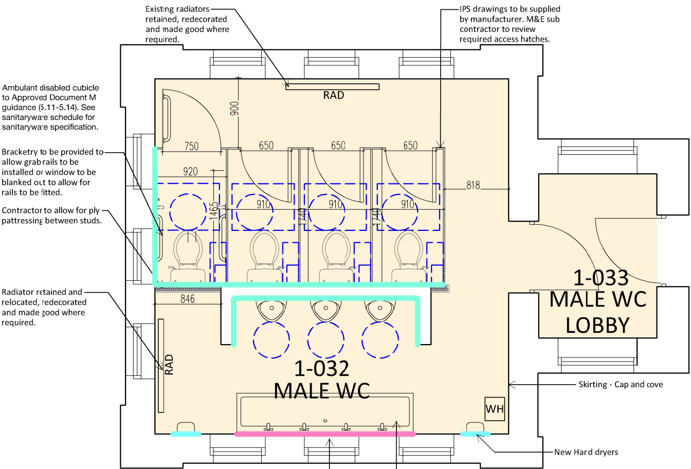
PROPOSED FINISHES PLAN - 1-032 WC
