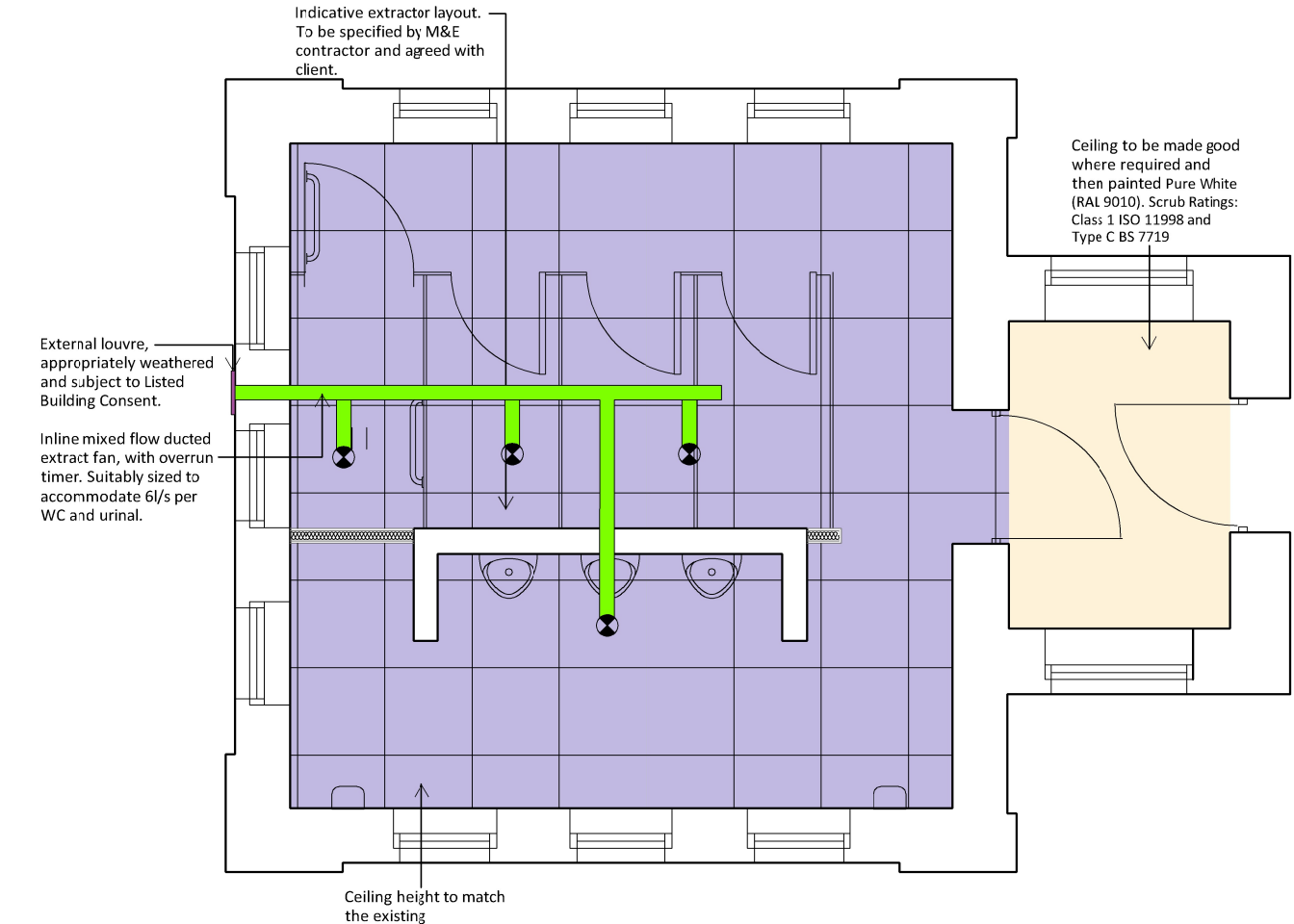
PROPOSED FINISHES PLAN - 1-032 WC
