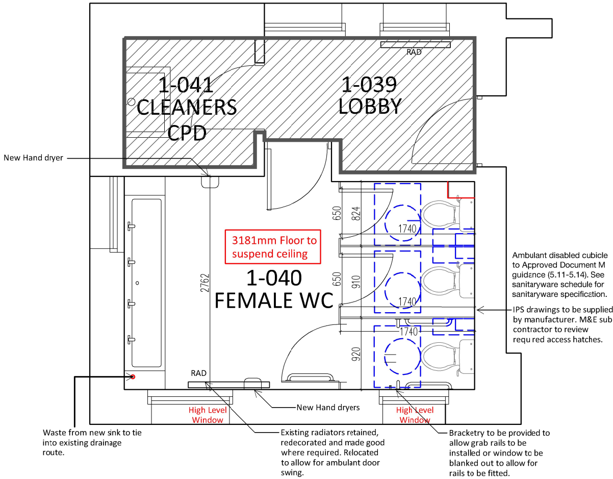
PROPOSED GENERAL ARRANGEMENT PLAN - 1-040 WC
