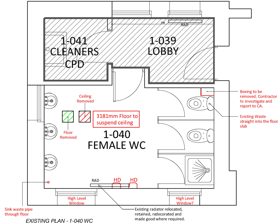
EXISTING PLAN - 1-040 WC
