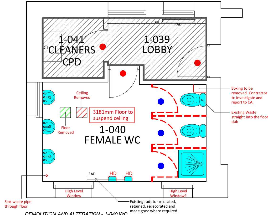
DEMOLITION AND ALTERATION - 1-040 WC
