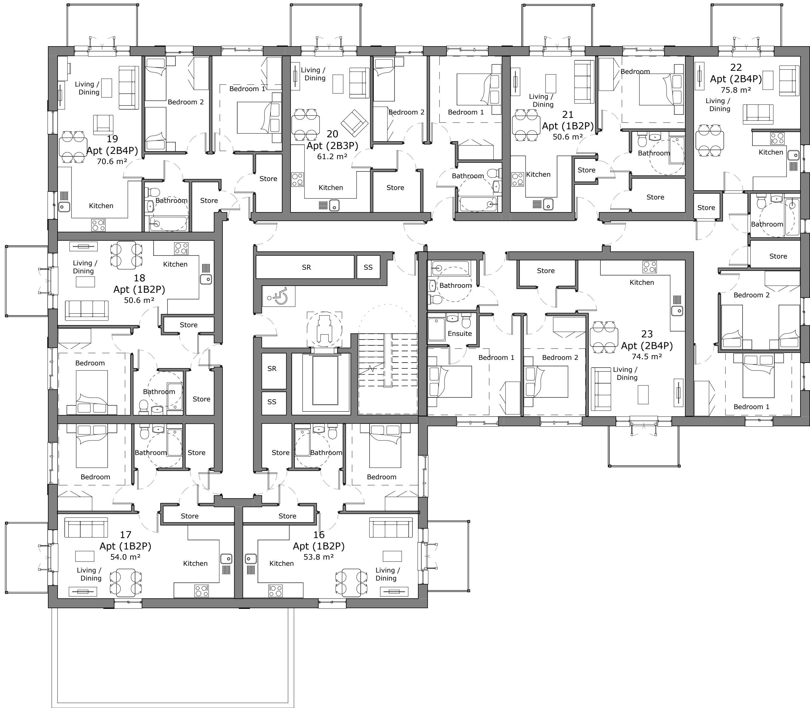
2nd Floor 1 : 100
