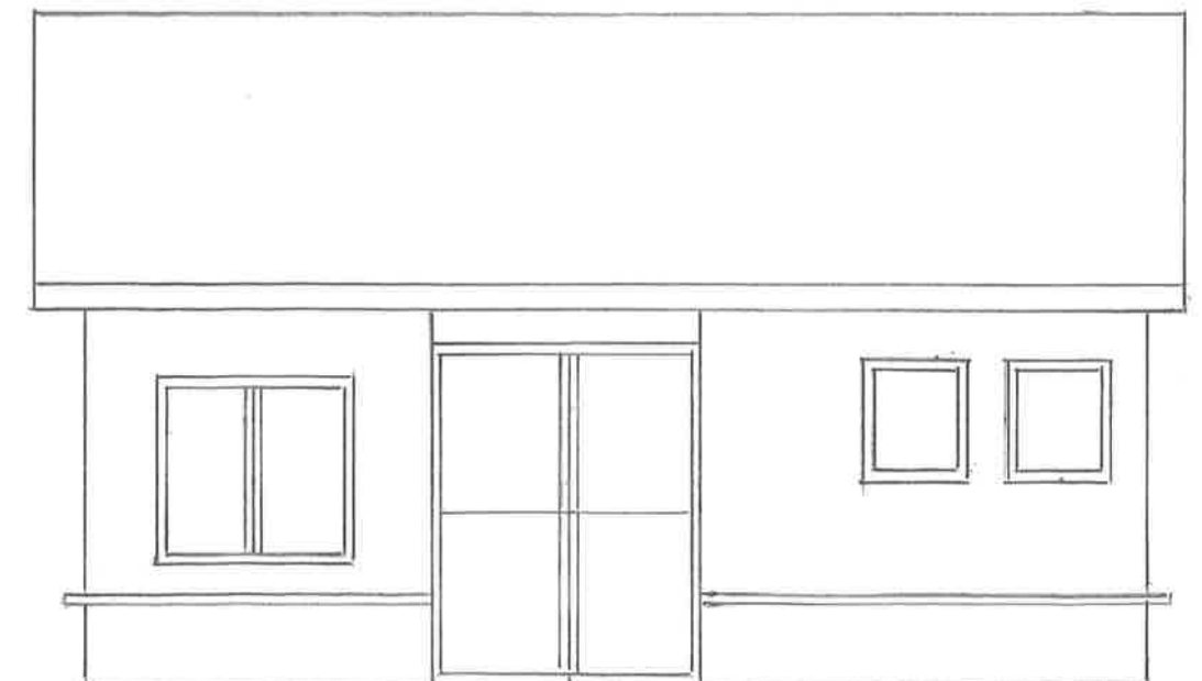
EXISTING NORTH SIDE ELEVATION 1:50
