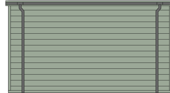
Rear (North-Eastern) Elevation
