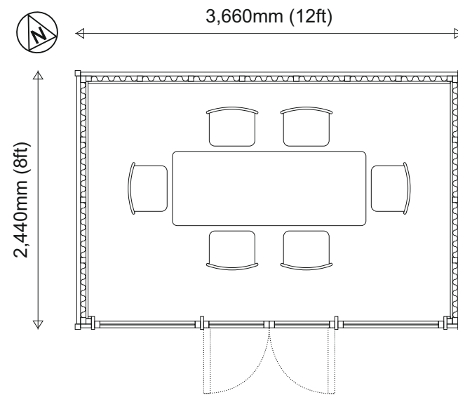
Floor Plan
