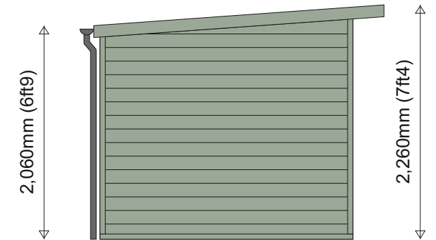
Side (North-West) Elevation
