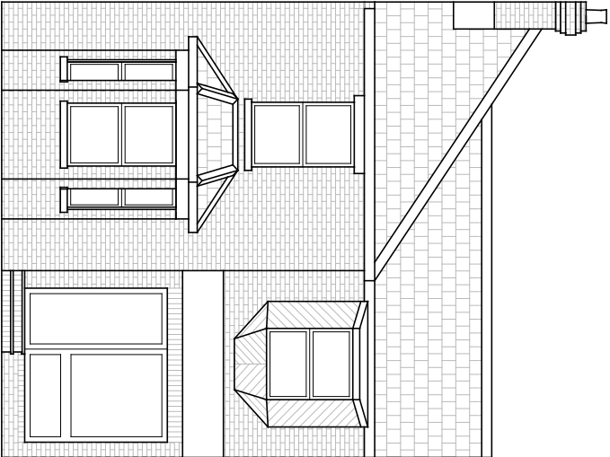
Existing Front (North) Elevation 1:100@A3
