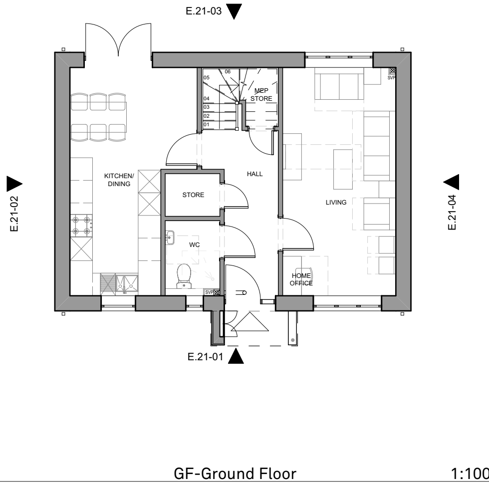
GF-Ground Floor
