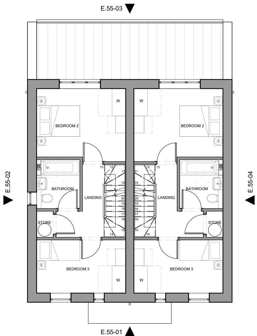
01-First Floor
