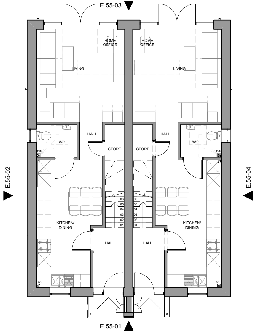
GF-Ground Floor
