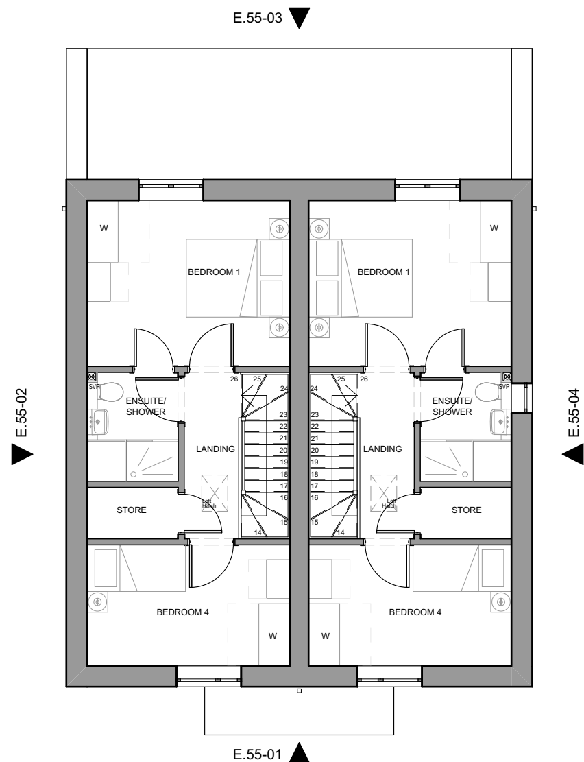
02-Second Floor
