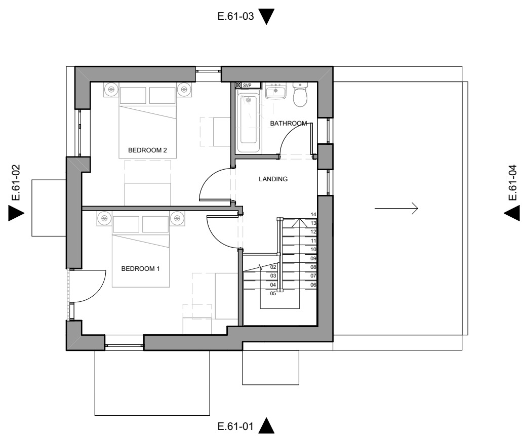
02-Second Floor
