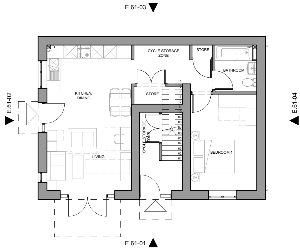
GF-Ground Floor
