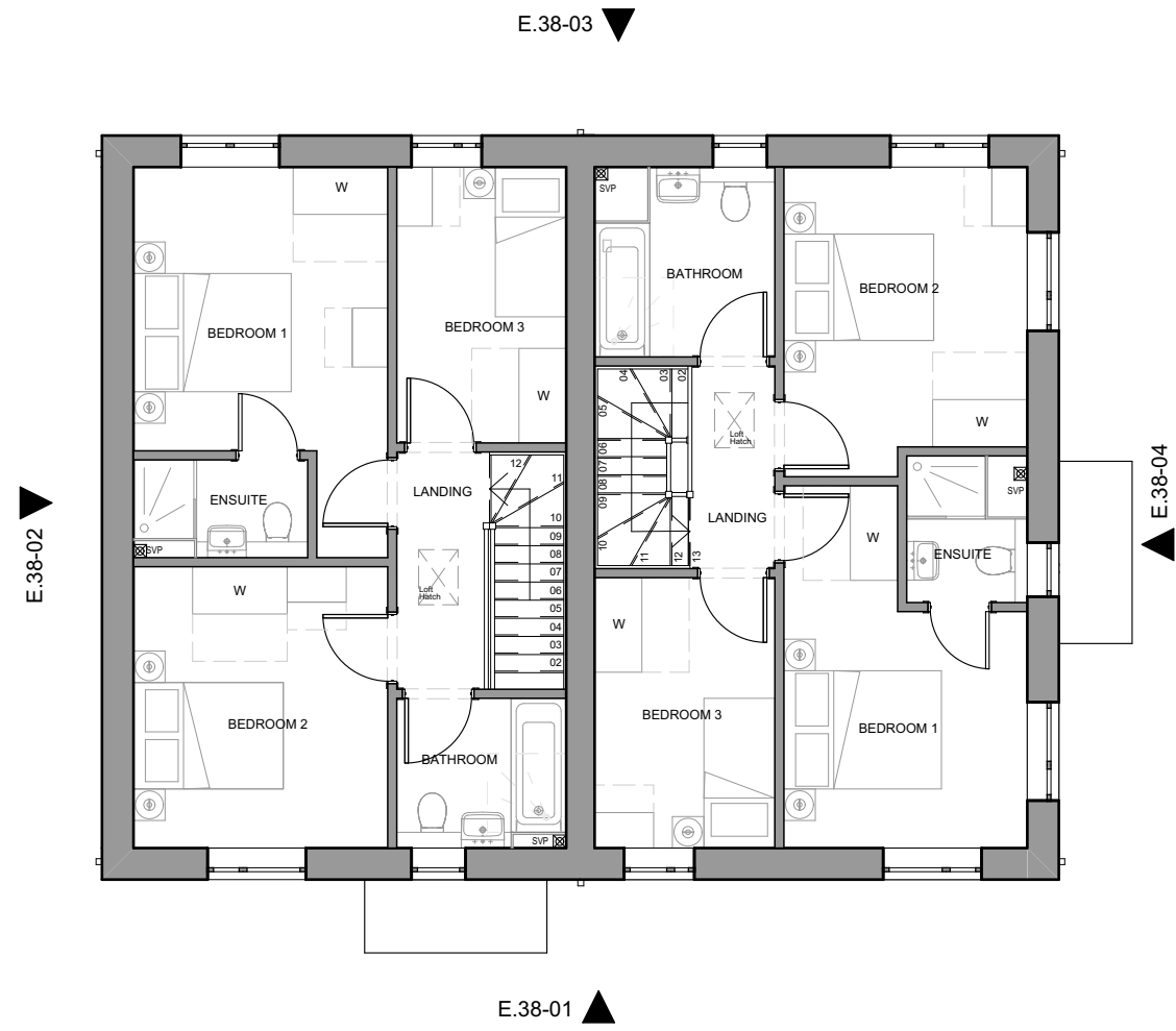
01-First Floor
