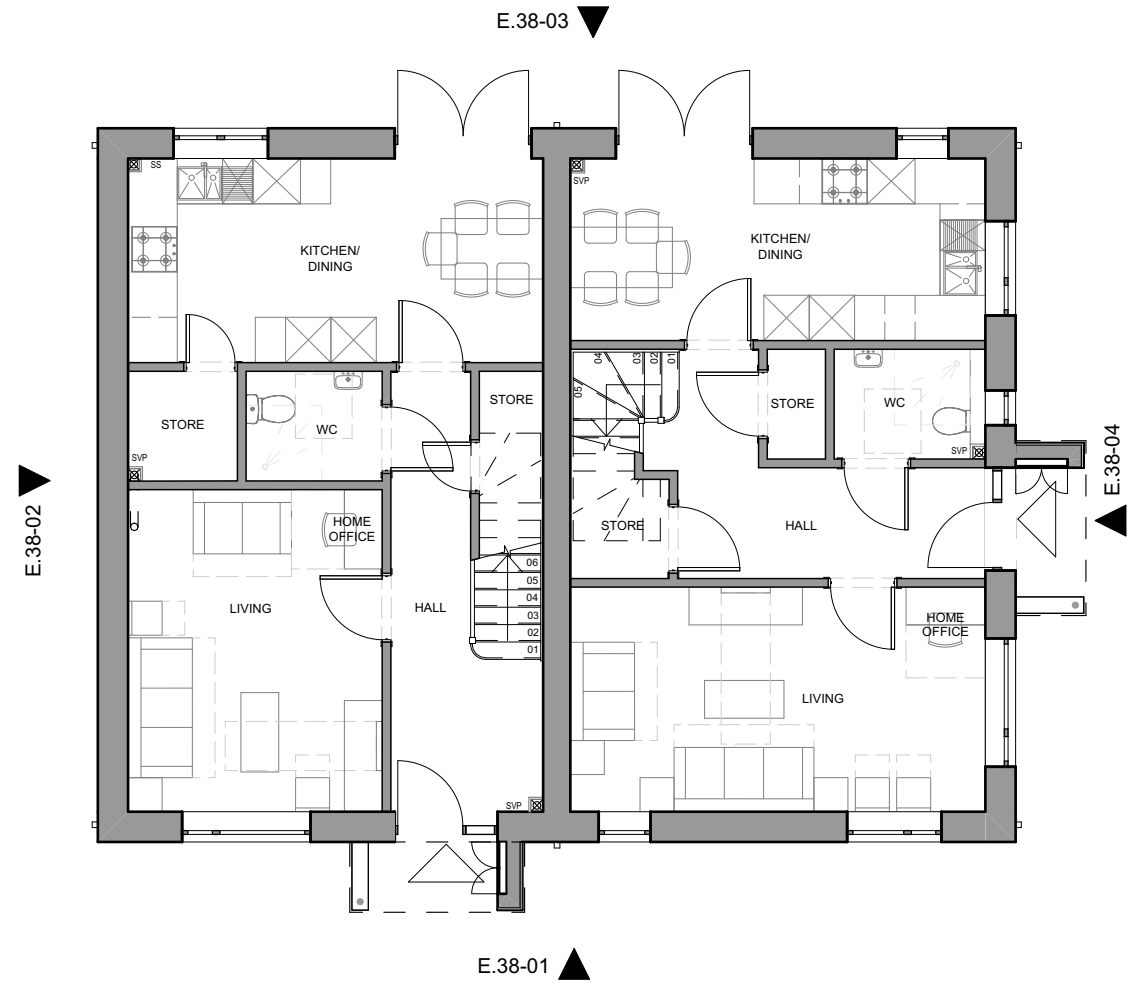
GF-Ground Floor
