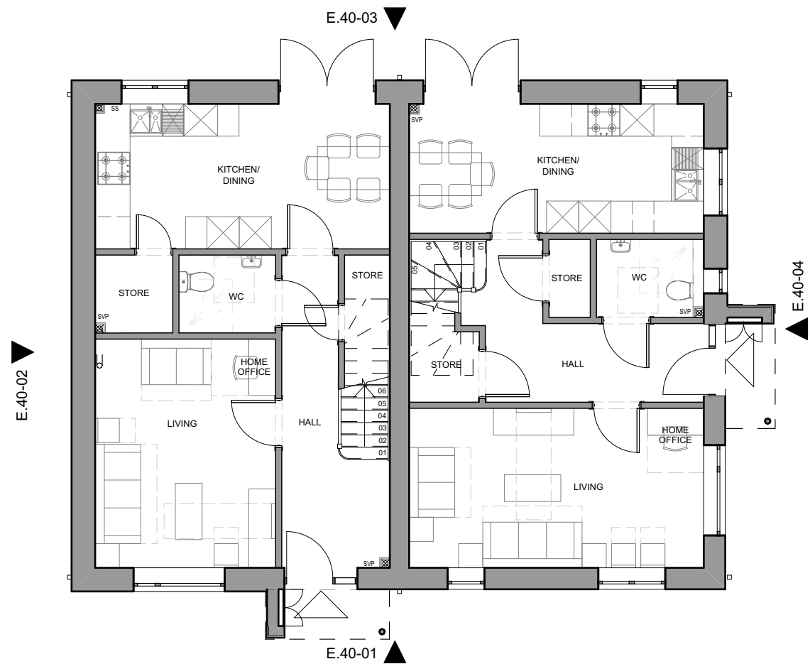
GF-Ground Floor
