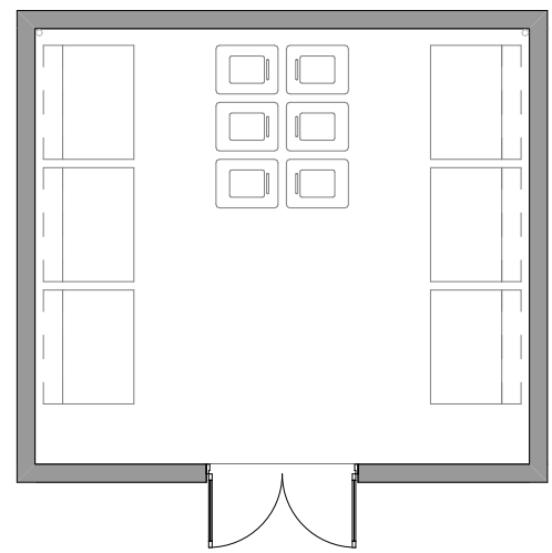
Type 3 Floor Plan 1:100
