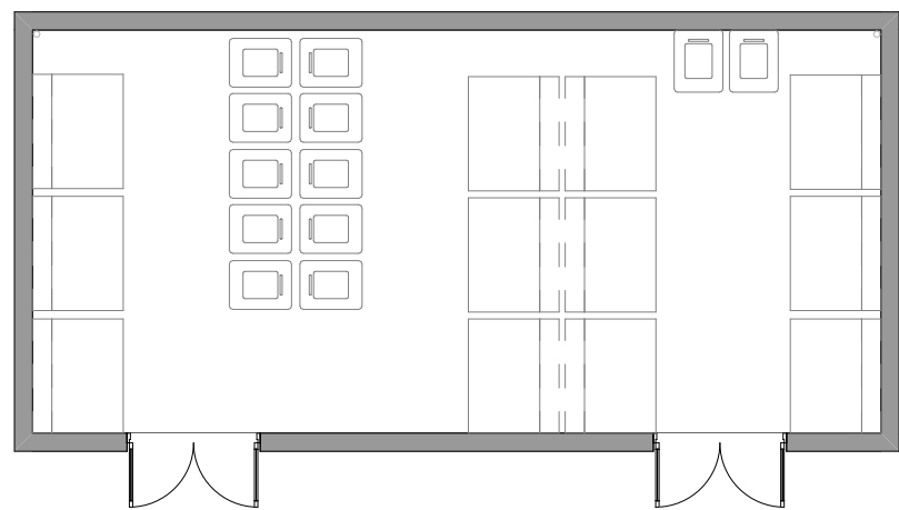
Type 5 Floor Plan 1:100
