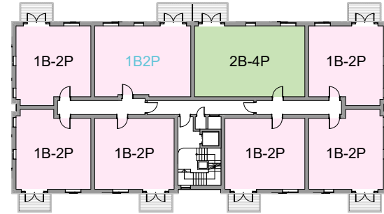
1:500 Second floor
