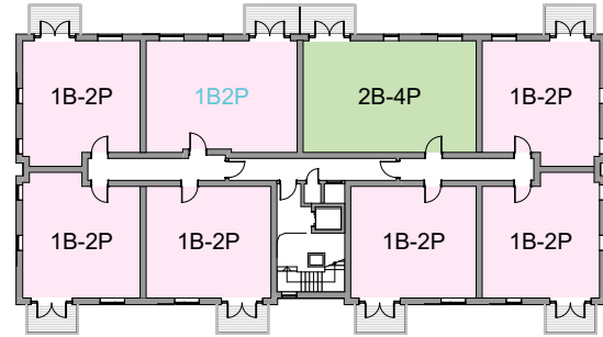
1:500 Third floor
