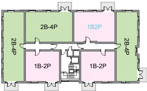
1:500 First floor
