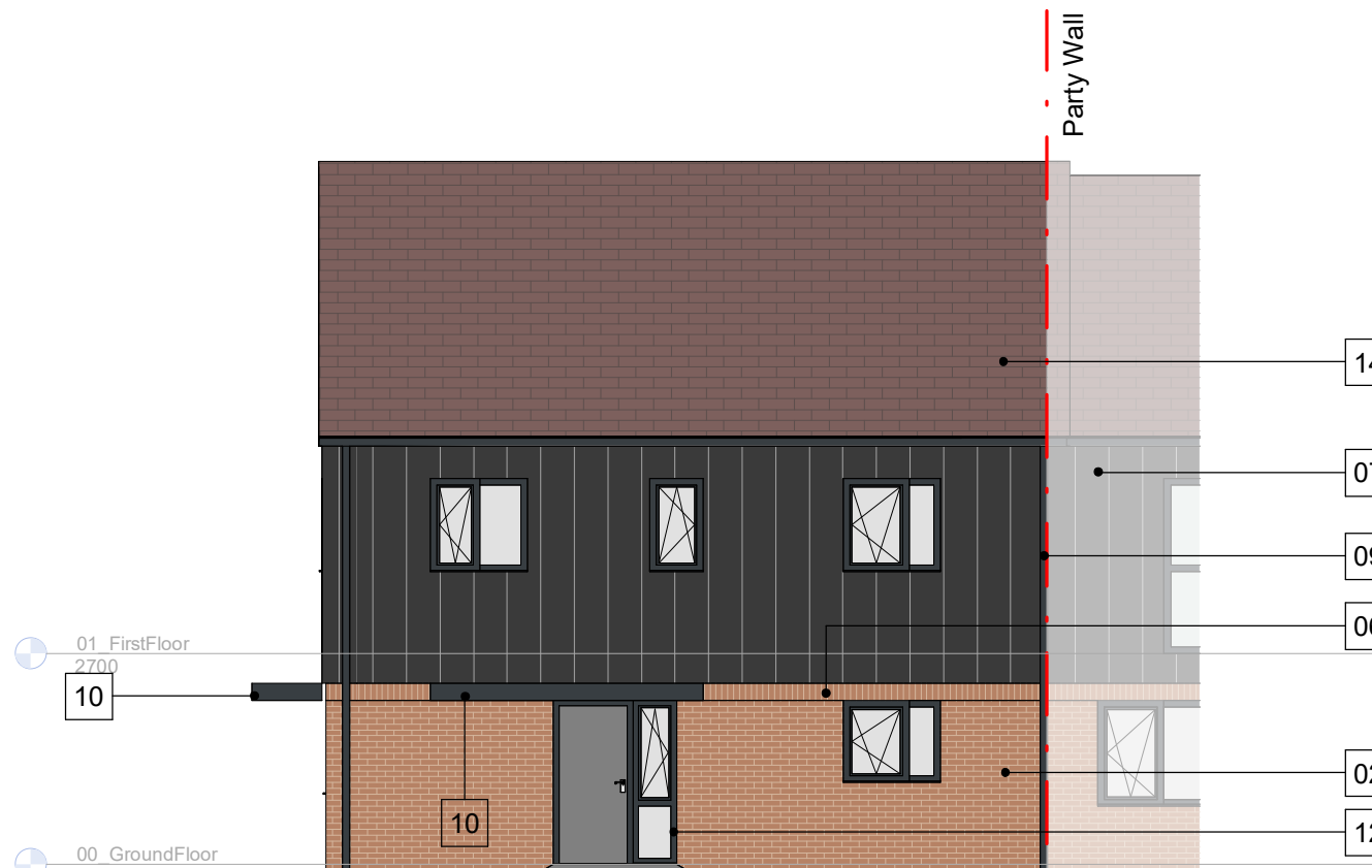
4 Front Elevation House Type M/N1
