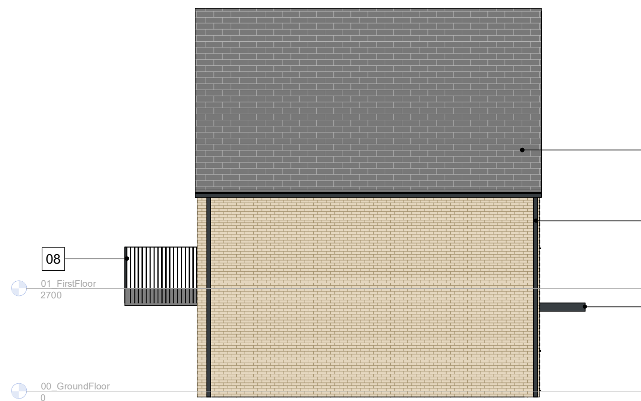
8 Left Side Elevation House Type M/N2
