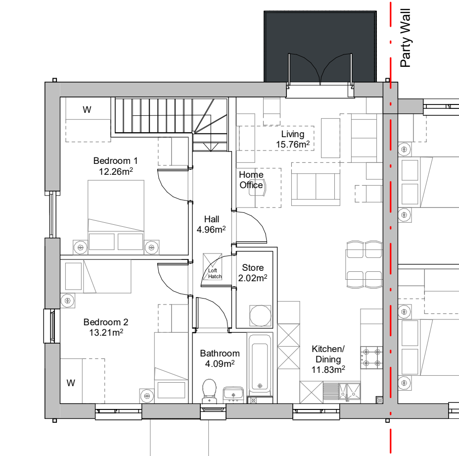
2 First Floor Plan
