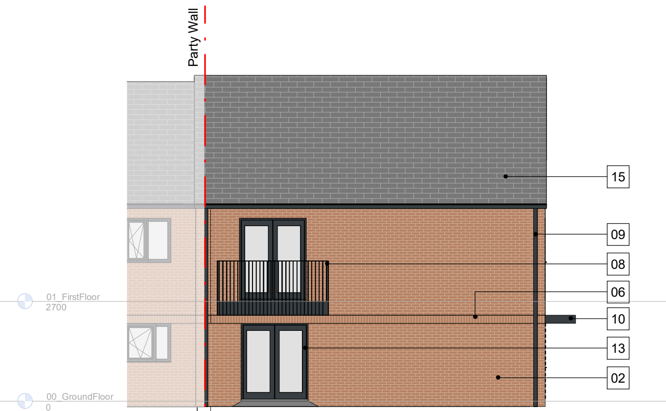
13 Rear Elevation House Type M/N3
