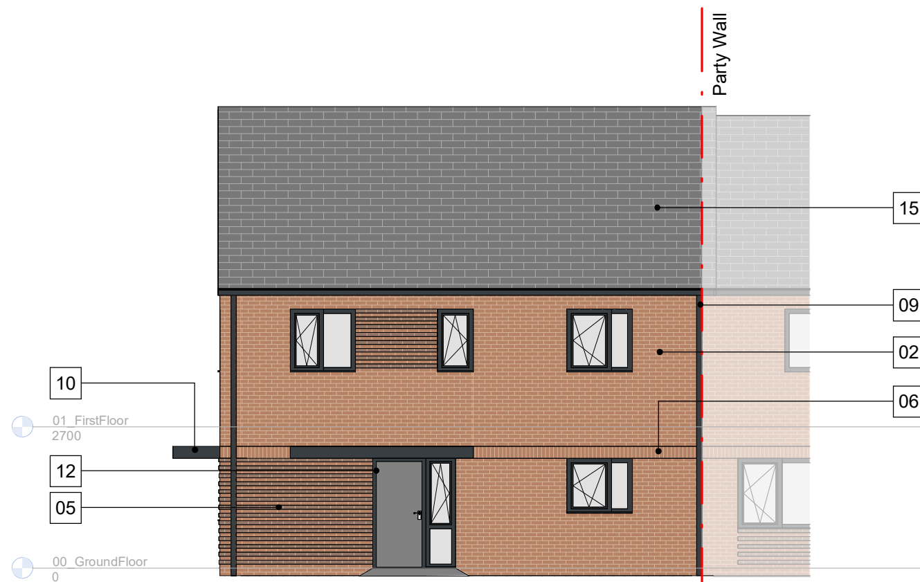
11 Front Elevation House Type M/N3
