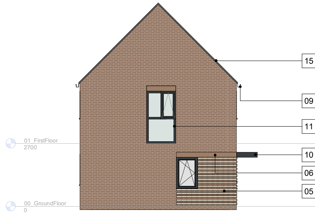
6 Left Side Elevation - House Type JJ
