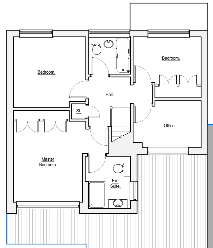
Proposed First Floor - 1:100
