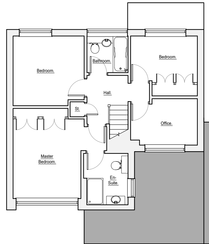
Existing First Floor - 1:100
