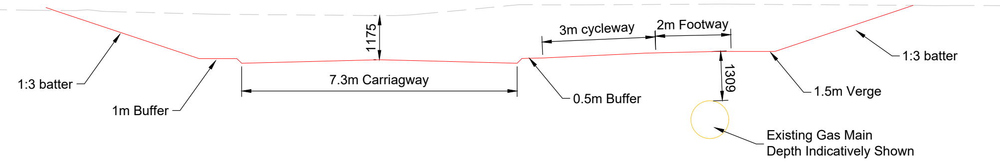
Section B-B Through Highway
