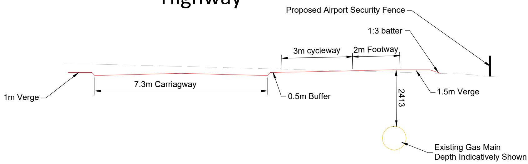
Section C-C Through Highway
