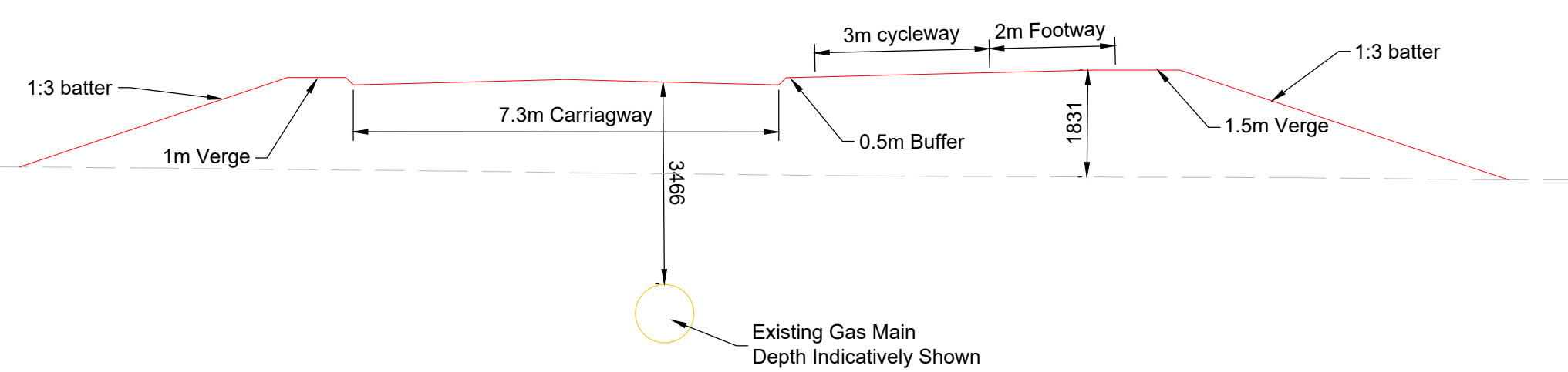
Section D-D Through Highway
