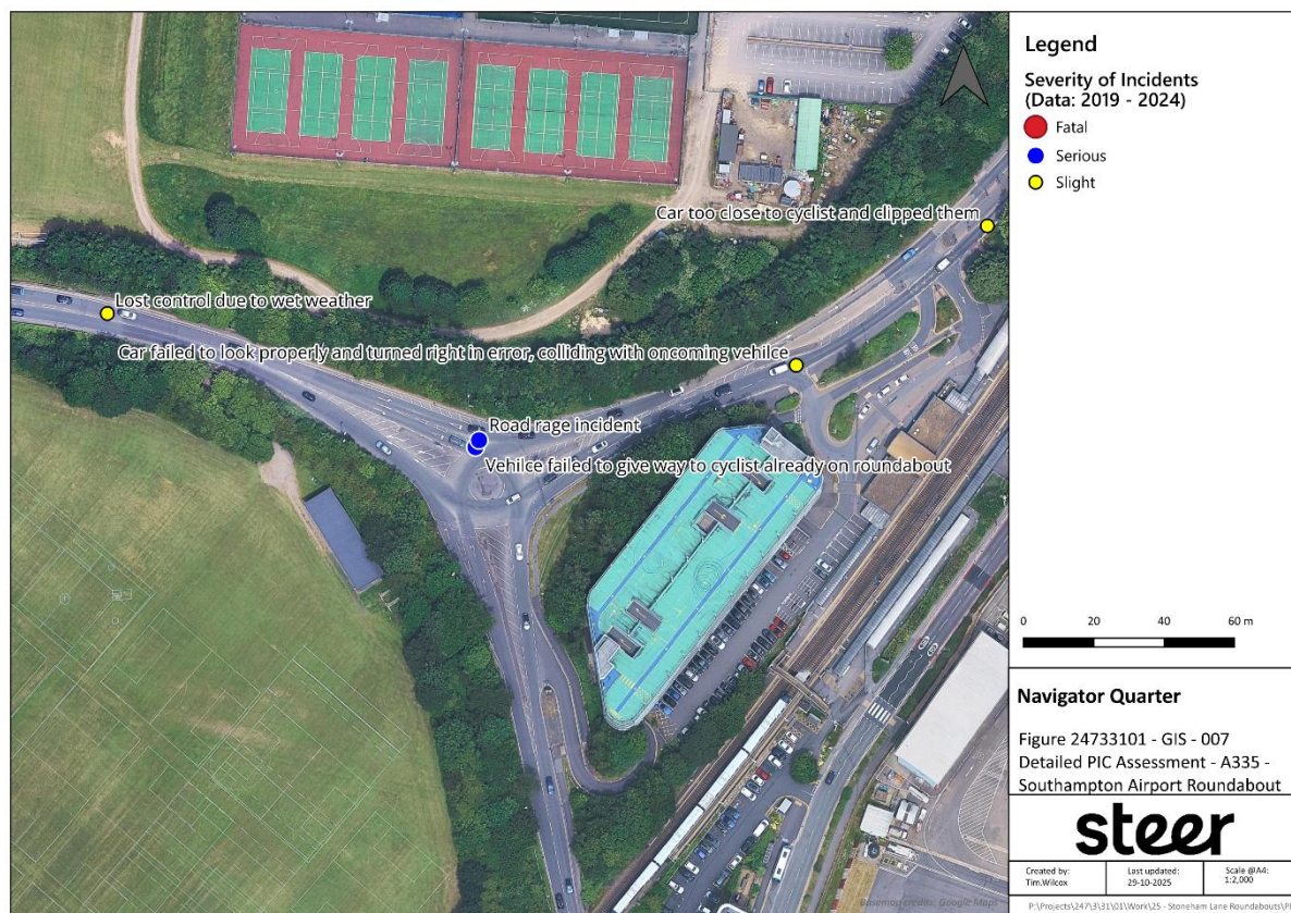
Figure 6: A335 Airport Roundabout PIC Analysis
