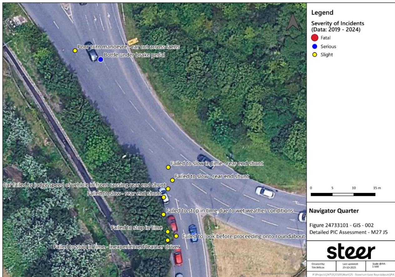
Figure 1: M27 Junction 5 PIC Analysis
