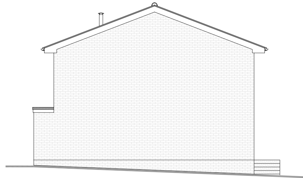
SIDE (SOUTHEAST) ELEVATION
