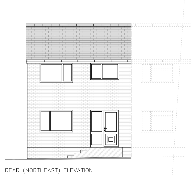
REAR (NORTHEAST) ELEVATION
