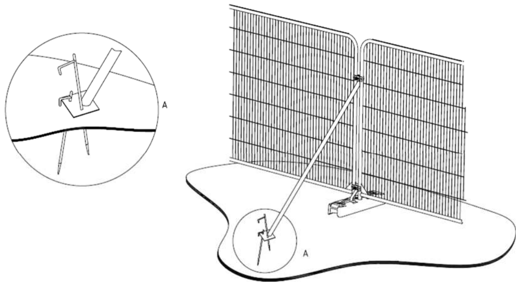
1 a) Stabilizer strut with base plate secured with ground pins
