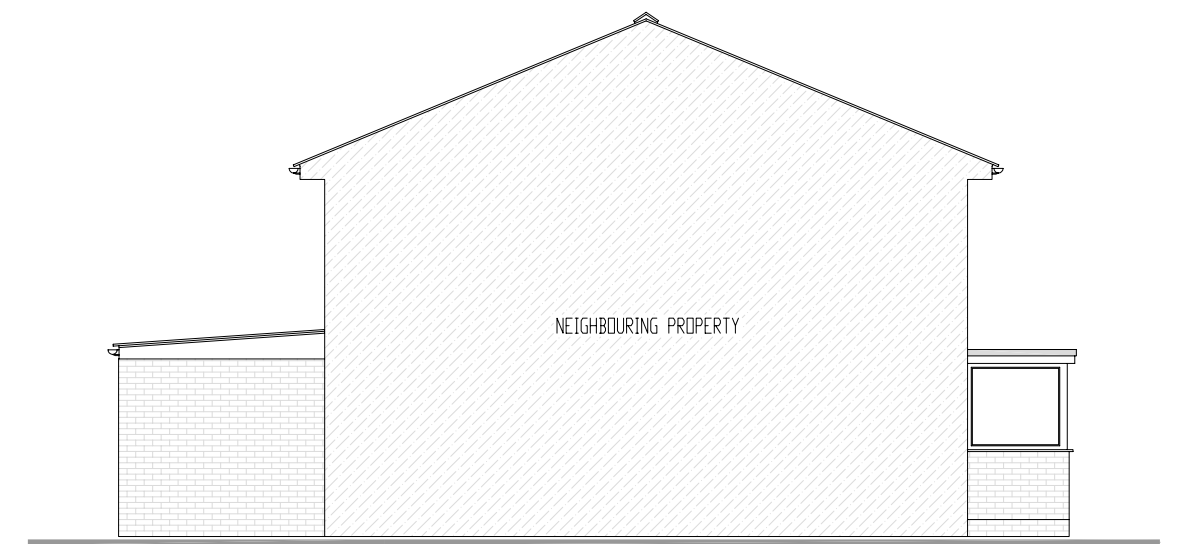
SIDE (NORTHWEST) ELEVATION
