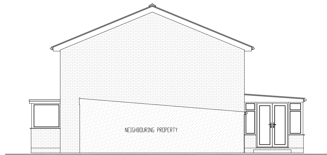
SIDE (SOUTHEAST) ELEVATION
