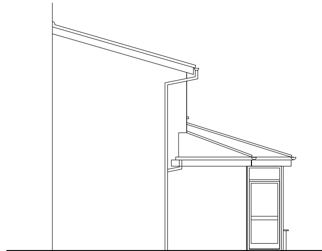
EXISTING NORTH WEST ELEVATION
